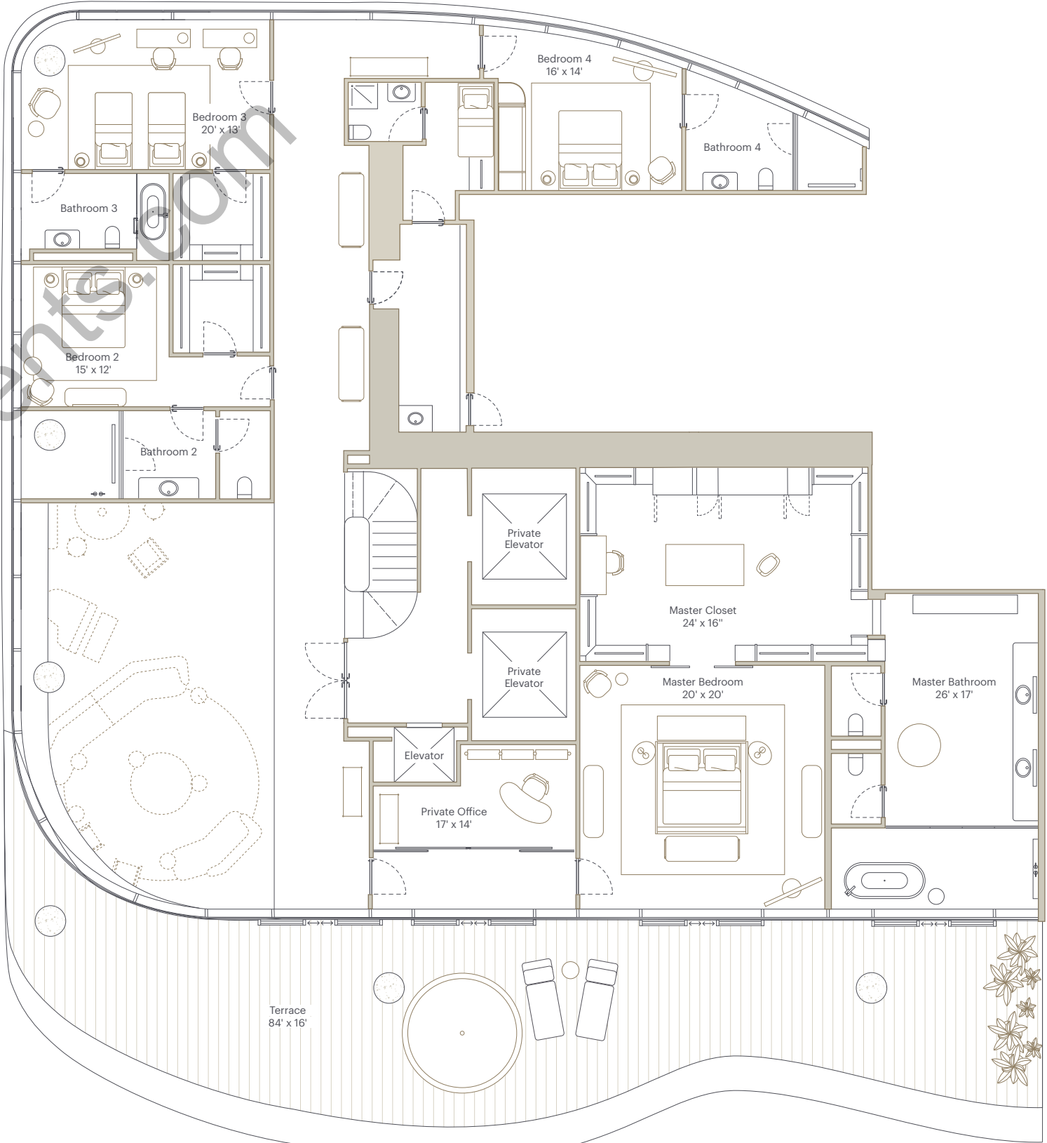
SECOND FLOOR
